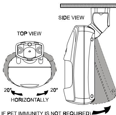
Figure 10. Tilt/Swivel Limits
