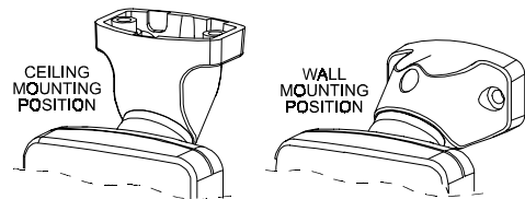
Figure 7. Wall and Ceiling Positions of Bracket
