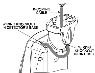
Figure 9. Routing the Cable
